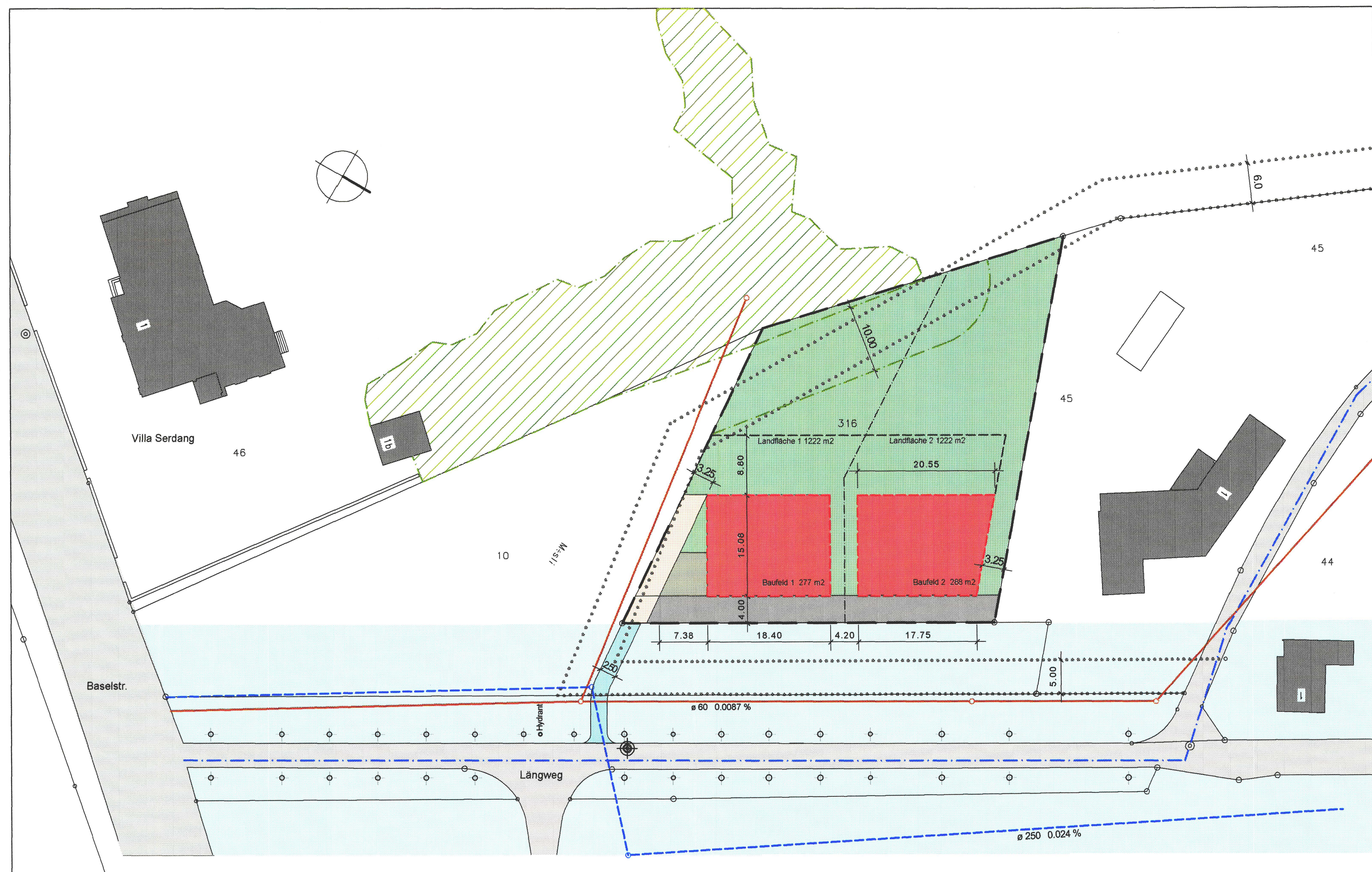
Situation M 1:500
