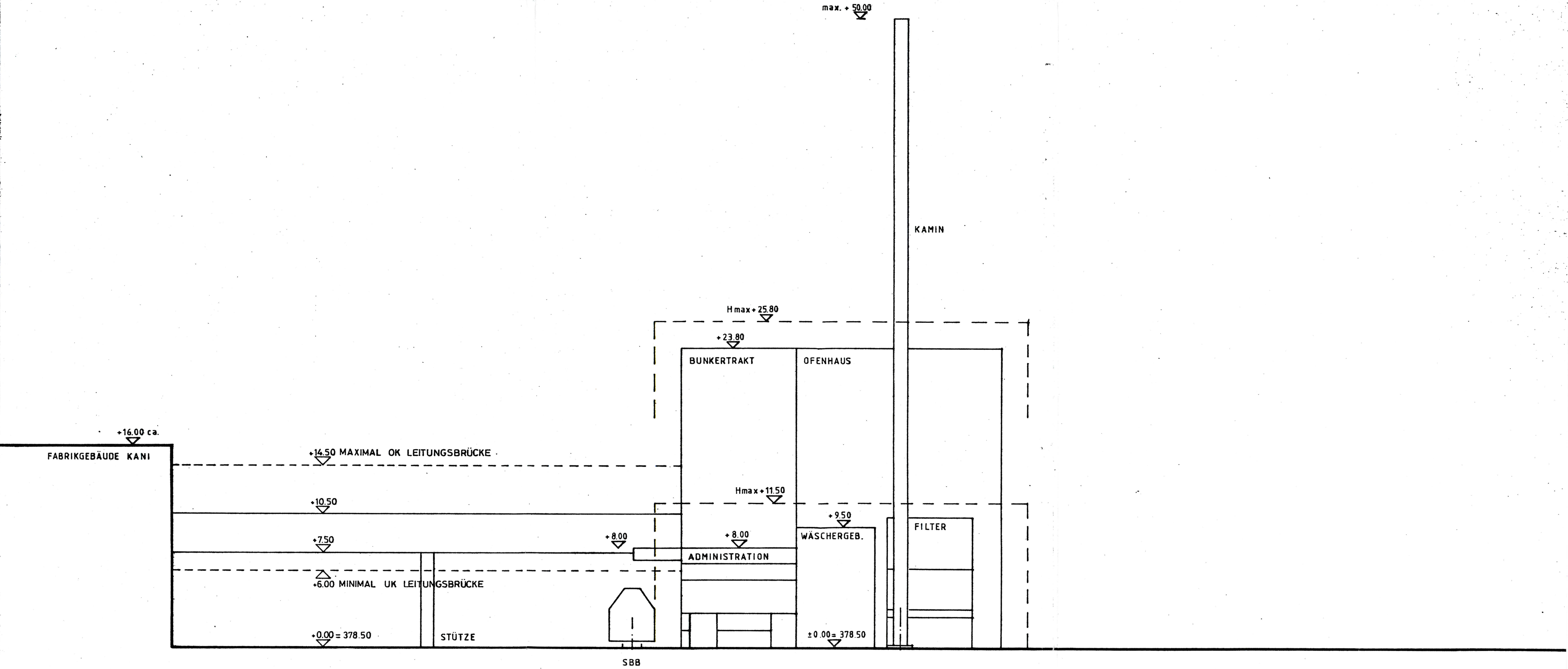
FASSADE WEST 1:200
